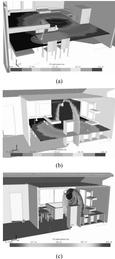
Fig. 9 Illumination field visualization in a house kitchen: two orthogonal thin slices of illuminance and colormaps, and illuminance isosurfaces
