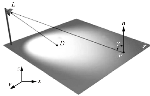
Fig. 3 Geometric information for illuminance field calculation
